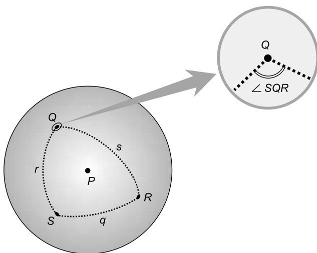
Fig. 11-6. The angle between two intersecting great-circle arcs, as considered within a circular region on the sphere so small that it is essentially a flat disk.
