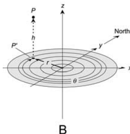
Fig. 6-3. (A) Mathematician's form of cylindrical coordinates for defining points in three-space. (B) Astronomer's and navigator's form of cylindrical coordinates for defining points in three-space.
