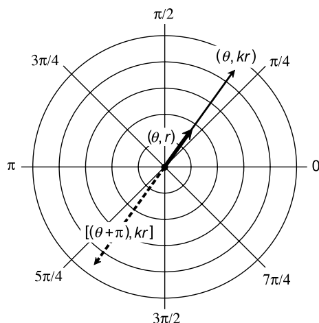
Fig. 6-8. Multiplication of a polar-plane vector a by a positive real scalar k , and by a negative real scalar -k . All angles are expressed in radians.
