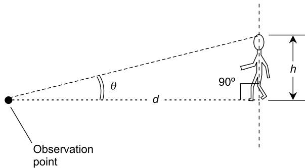
Fig. 8-4. Stadiometry requires that the height or width of a distant object be known.
