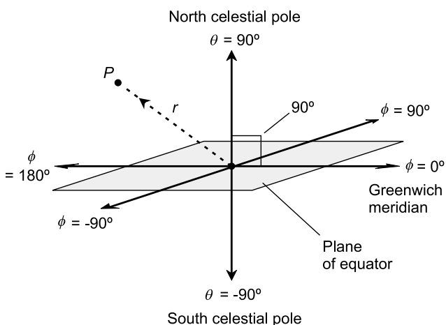
Fig. 6-4. (A) Spherical coordinates for defining points in three-space, where the angles \theta and \phi represent declination and right ascension, and r represents radius or range. (B) Spherical coordinates for defining points in three-space, where the angles \theta and \phi represent latitude and longitude, and r represents radius or range.
