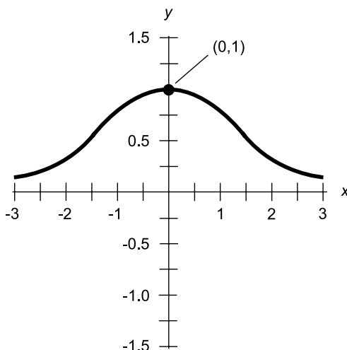
Fig. 4-5. Graph of the hyperbolic secant function.
