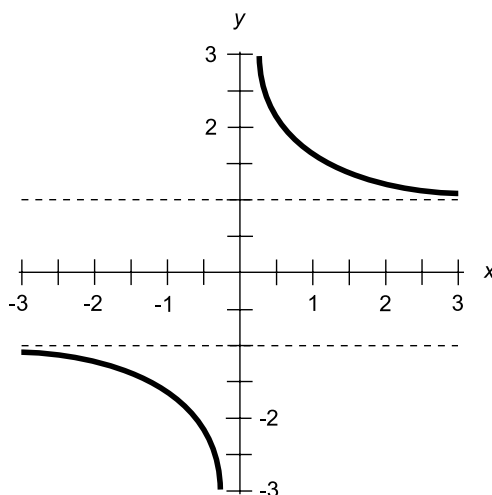
Fig. 4-6. Graph of the hyperbolic cotangent function.
