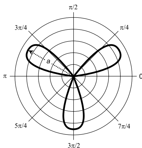
Fig. 5-8 (A) Polar graph of a three-leaved rose with equation r = a \cos 3\theta . (B) Polar graph of a three-leaved rose with equation r = a \sin 3\theta .
