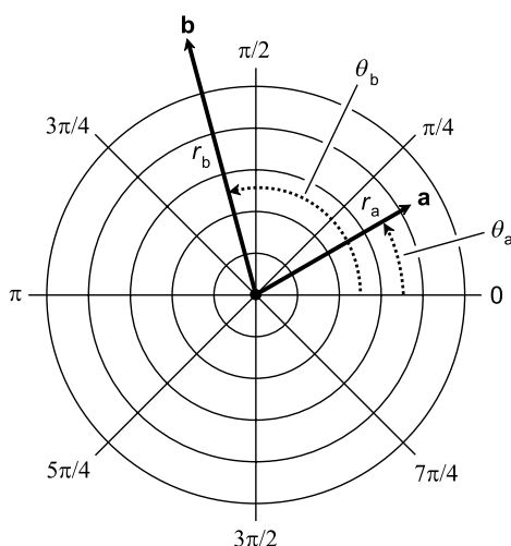
Fig. 6-7. Two vectors a and b in the polar plane. The angles are \theta_a and \theta_b . All angles are expressed in radians. The radii are r_a and r_b .
