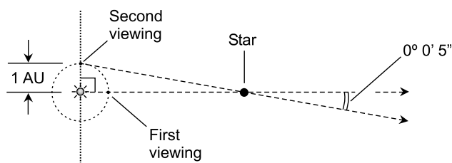
Fig. 8-6. Illustration for Problem 8-3.
