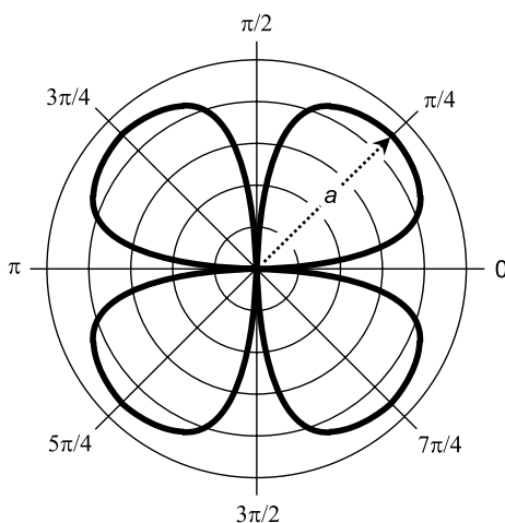
Fig. 5-9 (A) Polar graph of a four-leafed rose with equation r = a \cos 2\theta . (B) Polar graph of a four-leafed rose with equation r = a \sin 2\theta .
