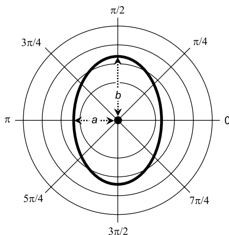
Fig. 5-5. Polar graph of an ellipse centered at the origin, with semi-axes a and b .
