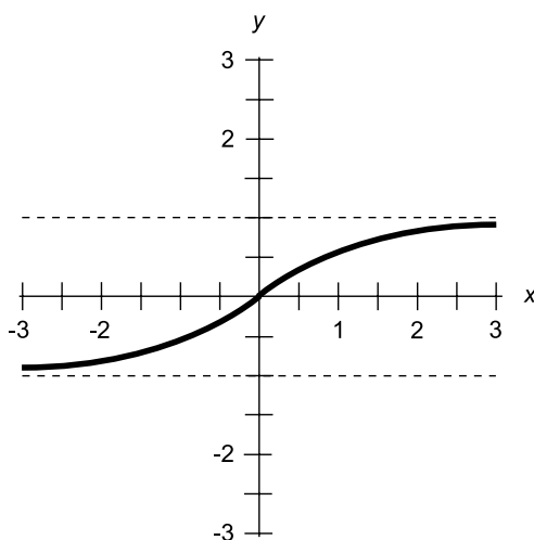
Fig. 4-3. Graph of the hyperbolic tangent function.
