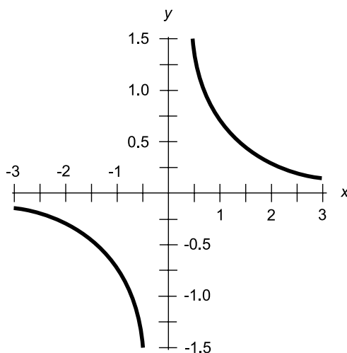
Fig. 4-4. Graph of the hyperbolic cosecant function.
