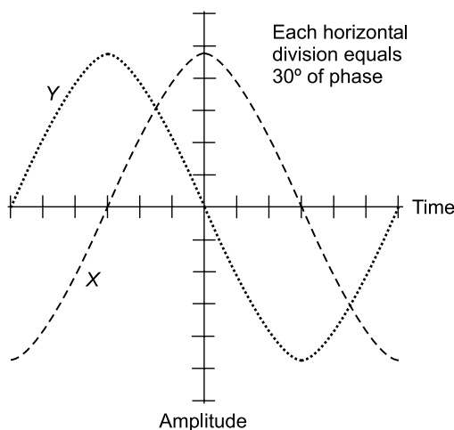
Fig. 9-6. Wave X lags wave Y by 90^\circ . Graphically, X appears displaced \frac{1}{4} cycle to the right of (later than) Y .
