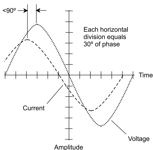
Fig. 9-11. An example of current that leads voltage by less than 90^\circ , as in a circuit containing resistance and capacitive reactance.
