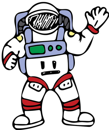
ASTRONAUT
