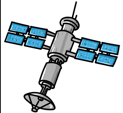
SATELLITE
