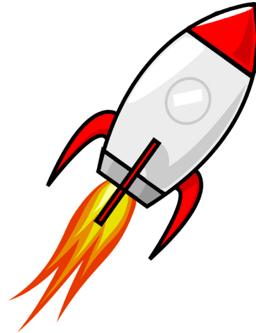
ROCKET
