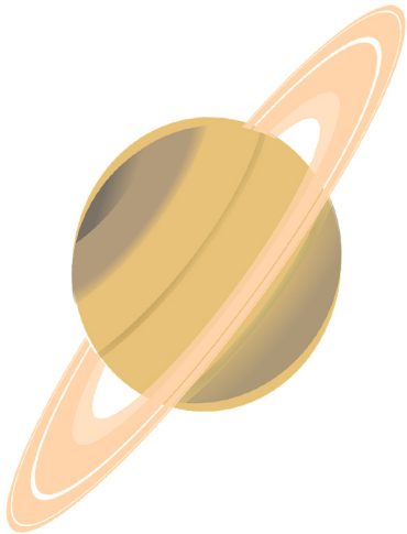
SATURN
