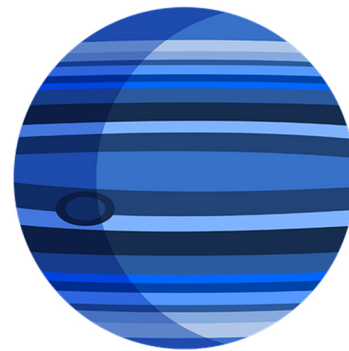
NEPTUNE
