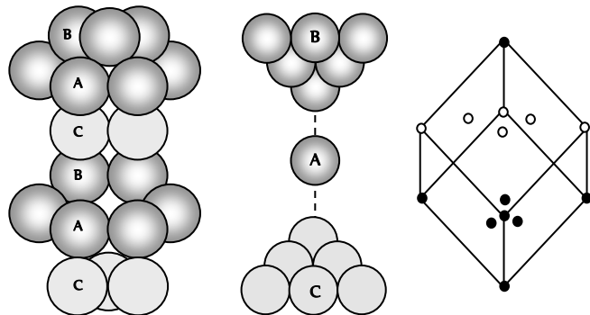
Fig. 5.10. Cubic close packing (ccp or fcc) in three dimensions
