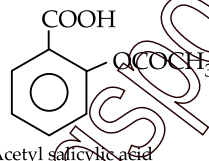
Acetyl salicylic acid
