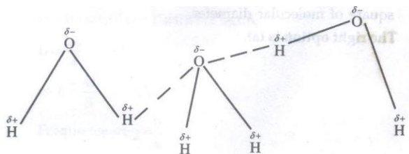
Fig. 3.16: Hydrogen bonding in water molecules
