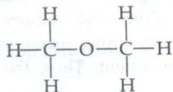
Fig. 2.19 Methoxy methane (Symmetrical ether)
