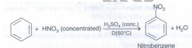
Fig. 1.20: Making Nitrobenzene
