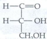
Fig. 2.20: D(+)-Glyceraldehyde
