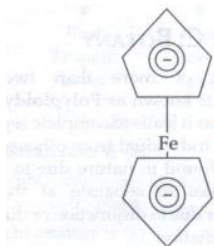
Fig. 4.31: Ferrocene ( \text{Fe}(\eta^5\text{-C}_5\text{H}_5)_2 )
