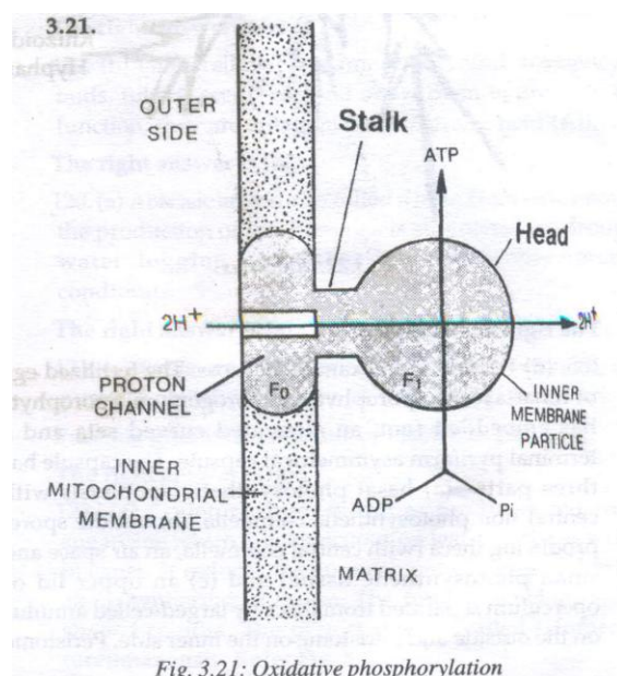
Fig. 3.21: Oxidative phosphorylation
