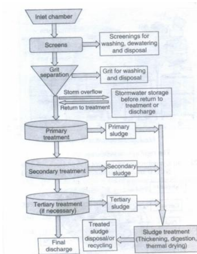
Fig. 1.52: Activated sludge treatment
