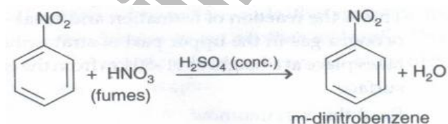
Fig. 1.21: Making m-dinitrobenzene
