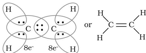
C_2H_4 molecule
