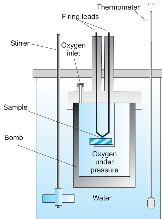
Fig. 6.7 Bomb calorimeter
