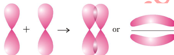
p-orbital p-orbital p-p overlapping
