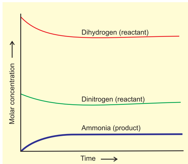
Fig 7.4 Depiction of equilibrium for the reaction N_2(g) + 3H_2(g) \rightleftharpoons 2NH_3(g)
