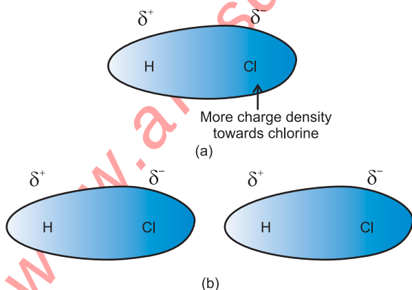
Fig. 5.2 (a) Distribution of electron cloud in HCl a polar molecule, (b) Dipole-dipole interaction between two polar molecules
