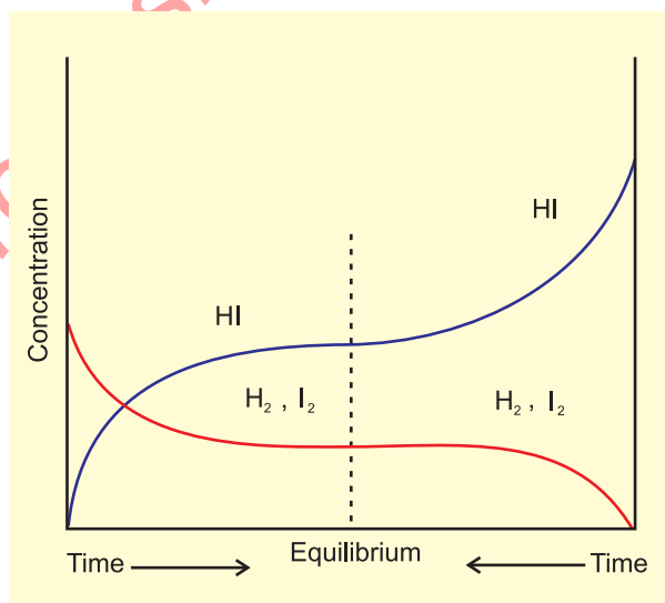
Fig.7.5 Chemical equilibrium in the reaction H_2(g) + I_2(g) \rightleftharpoons 2HI(g) can be attained from either direction
