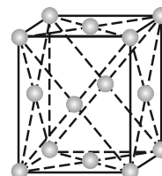
Face-centred
