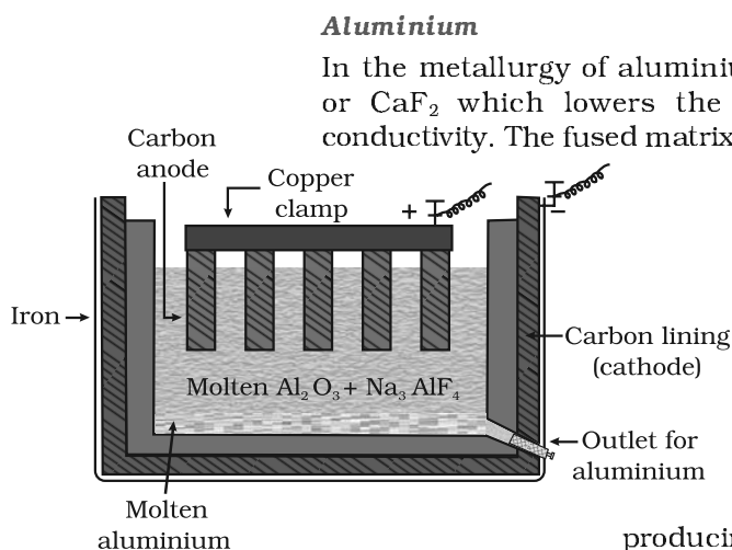
Fig. 6.6: Electrolytic cell for the extraction of aluminium
