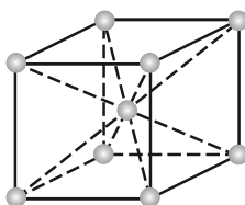
Body-centred
