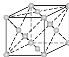
Face-centred
