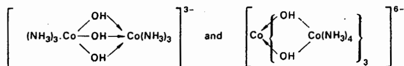
Figure 7.31 Polymerization isomers.
