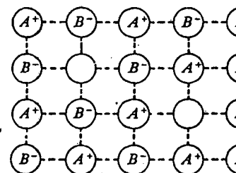
Figure 3.13 Schottky defect.
