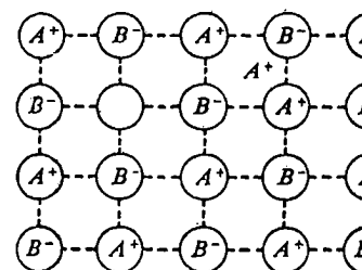
Figure 3.14 Frenkel defect.
