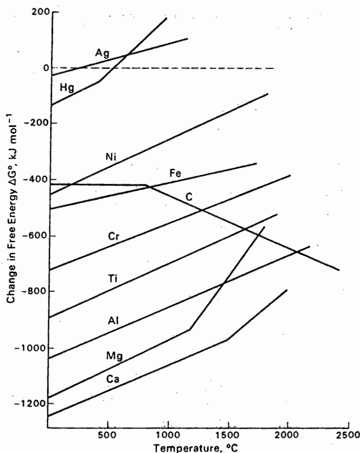
Figure 6.5 Ellingham diagram showing the change in free energy \Delta G with temperature for oxides (based on 1 g mol of oxygen in each case).
