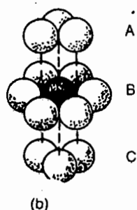
Figure 2.5 Arrangement of 12 neighbours in hexagonal and cubic close-packed structures. (a) Hexagonal close-packed. (b) Cubic close-packed. (Note that the top and bottom layers are the same, and the middle layer is rotated 60° relative to the other two layers.)
