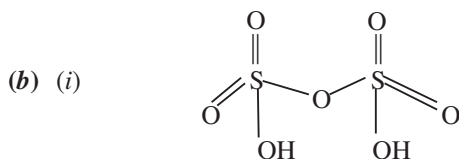
H_2S_2O_7 (Pyrosulphuric acid)
