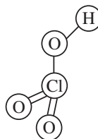
Chloric acid ( \text{HClO}_4 )
