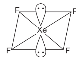
\text{XeF}_4 (Square planar)
