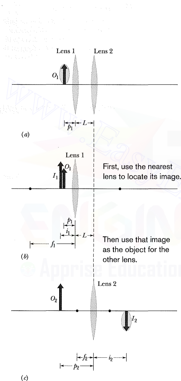
Fig. 34-18 (a) Seed O_1 is distance p_1 from a two-lens system with lens separation L . We use the arrow to orient the seed. (b) The image I_1 produced by lens 1 alone. (c) Image I_1 acts as object O_2 for lens 2 alone, which produces the final image I_2 .
