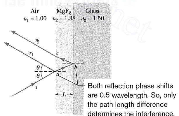
Fig. 35-19 Unwanted reflections from glass can be suppressed (at a chosen wavelength) by coating the glass with a thin transparent film of magnesium fluoride of the properly chosen thickness.
