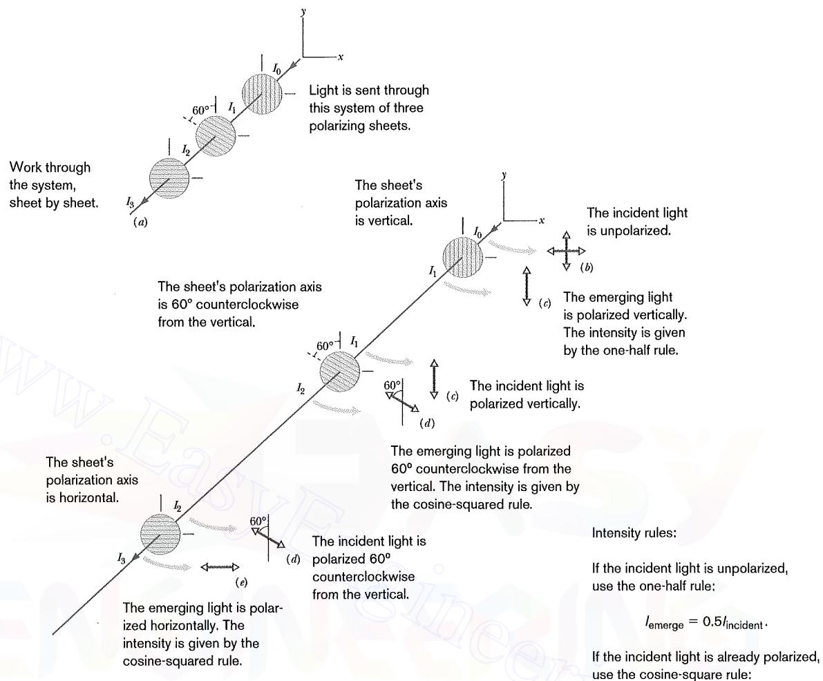
Fig. 33-15 (a) Initially unpolarized light of intensity I_0 is sent into a system of three polarizing sheets. The intensities I_1 , I_2 , and I_3 of the light transmitted by the sheets are labeled. Shown also are the polarizations, from head-on views, of (b) the initial light and the light transmitted by (c) the first sheet, (d) the second sheet, and (e) the third sheet.
