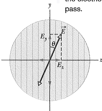
Fig. 33-12 Polarized light approaching a polarizing sheet. The electric field \vec{E} of the light can be resolved into components E_y (parallel to the polarizing direction of the sheet) and E_z (perpendicular to that direction). Component E_y will be transmitted by the sheet; component E_z will be absorbed.
