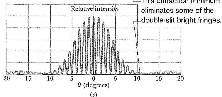
Fig. 36-15 (a) The intensity plot to be expected in a double-slit interference experiment with vanishingly narrow slits. (b) The intensity plot for diffraction by a typical slit of width a (not vanishingly narrow). (c) The intensity plot to be expected for two slits of width a . The curve of (b) acts as an envelope, limiting the intensity of the double-slit fringes in (a). Note that the first minima of the diffraction pattern of (b) eliminate the double-slit fringes that would occur near 12^\circ in (c).
