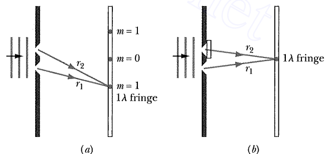
Fig. 35-11 (a) Arrangement for two-slit interference (not to scale). The locations of three bright fringes (or maxima) are indicated. (b) A strip of plastic covers the top slit. We want the 1\lambda fringe to be at the center of the pattern.
