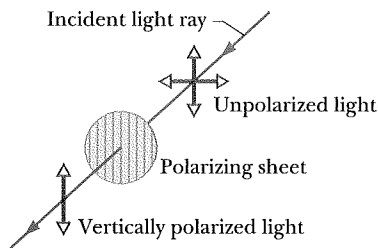
Fig. 33-11 Unpolarized light becomes polarized when it is sent through a polarizing sheet. Its direction of polarization is then parallel to the polarizing direction of the sheet, which is represented here by the vertical lines drawn in the sheet.
