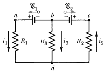
Fig. 27-9 A multiloop circuit consisting of three branches: left-hand branch bad , right-hand branch bcd , and central branch bd . The circuit also consists of three loops: left-hand loop badb , right-hand loop bcd b , and big loop badcb .
