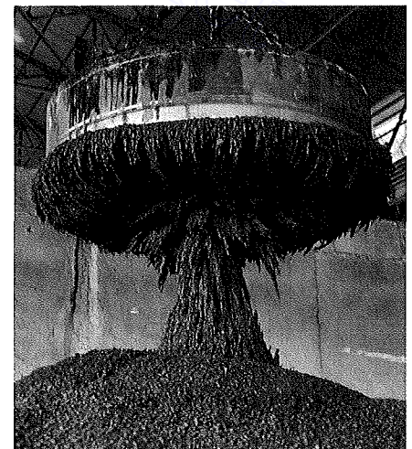
Fig. 28-1 Using an electromagnet to collect and transport scrap metal at a steel mill. (Digital Vision/Getty Images)
