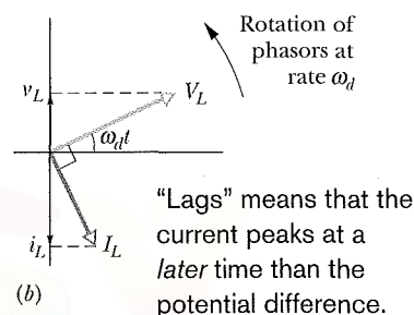
Fig. 31-13 (a) The current in the inductor lags the voltage by 90^\circ (= \pi/2 \text{ rad}) . (b) A phasor diagram shows the same thing.
