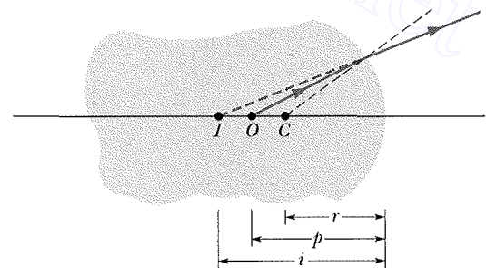
Fig. 34-13 A piece of amber with a mosquito from the Jurassic period, with the head buried at point O. The spherical refracting surface at the right end, with center of curvature C, provides an image I to an observer intercepting rays from the object at O.
