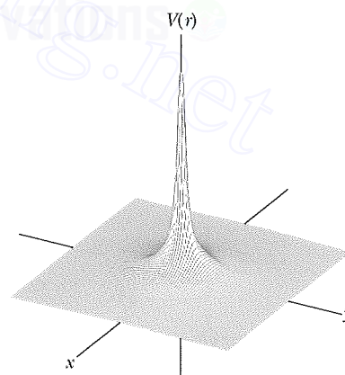
Fig. 24-7 A computer-generated plot of the electric potential V(r) due to a positive point charge located at the origin of an xy plane. The potentials at points in the xy plane are plotted vertically. (Curved lines have been added to help you visualize the plot.) The infinite value of V predicted by Eq. 24-26 for r = 0 is not plotted.
