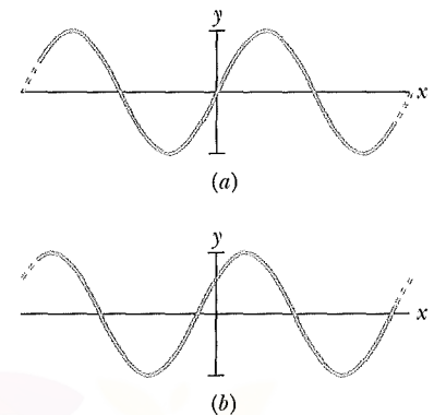
Fig. 16-6 A sinusoidal traveling wave at t = 0 with a phase constant \phi of (a) 0 and (b) \pi/5 rad.
