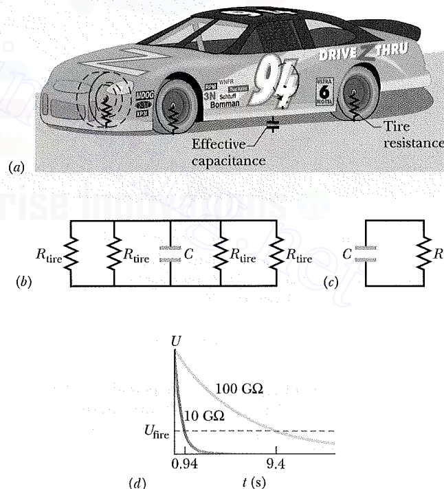
Fig. 27-17 (a) A charged car and the pavement acts like a capacitor that can discharge through the tires. (b) The effective circuit of the car–pavement capacitor, with four tire resistances R_{\text{tire}} connected in parallel. (c) The equivalent resistance R of the tires. (d) The electric potential energy U in the car–pavement capacitor decreases during discharge.
