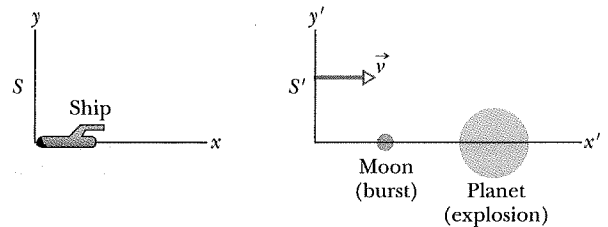
Fig. 37-10 A planet and its moon in reference frame S' move rightward with speed v relative to a starship in reference frame S .
