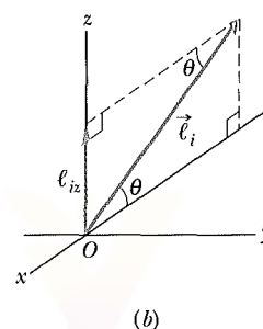
Fig. 11-15 (a) A rigid body rotates about a z axis with angular speed \omega . A mass element of mass \Delta m_i within the body moves about the z axis in a circle with radius r_{\perp i} . The mass element has linear momentum \vec{p}_i , and it is located relative to the origin O by position vector \vec{r}_i . Here the mass element is shown when r_{\perp i} is parallel to the x axis. (b) The angular momentum \vec{\ell}_i with respect to O , of the mass element in (a). The z component \ell_{iz} is also shown.
