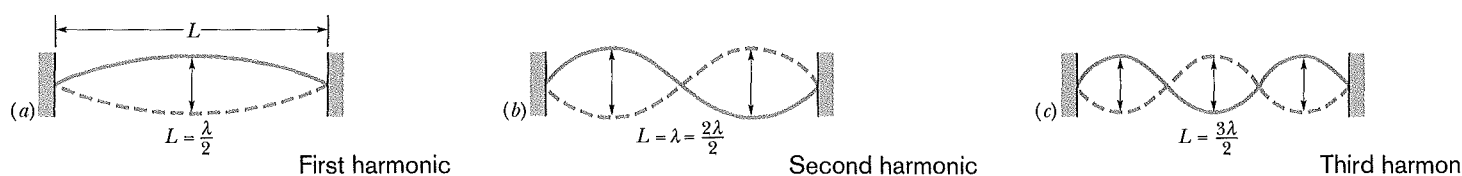
Fig. 16-20 A string, stretched between two clamps, is made to oscillate in standing wave patterns. (a) The simplest possible pattern consists of one loop , which refers to the composite shape formed by the string in its extreme displacements (the solid and dashed lines). (b) The next simplest pattern has two loops. (c) The next has three loops.
