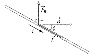
Fig. 28-16 A wire carrying current i makes an angle \phi with magnetic field \vec{B} . The wire has length L in the field and length vector \vec{L} (in the direction of the current). A magnetic force \vec{F}_B = i\vec{L} \times \vec{B} acts on the wire.
