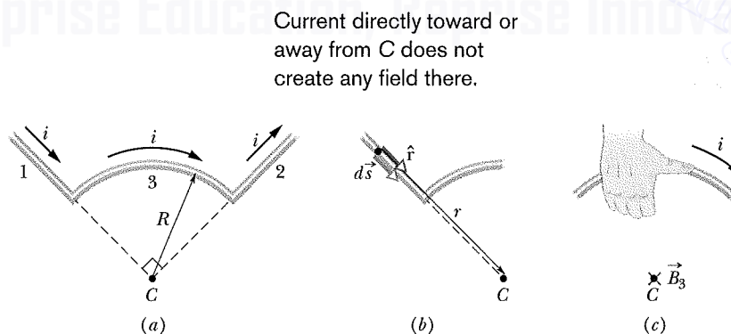
Fig. 29-7 (a) A wire consists of two straight sections (1 and 2), and carries current i . (b) For a current-length element in section 1, the angle between d\vec{s} and \hat{r} is zero. (c) Determining the direction of magnetic field \vec{B}_3 at C due to the current in the circular arc; the field is into the page there.
