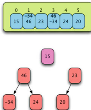
Fig. 9.20 After Forming a Second Sub-Heap
