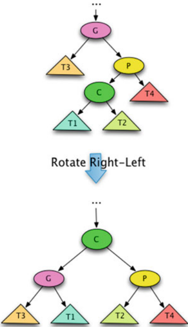
Fig. 10.12 Splay Tree Right-Left Rotate
