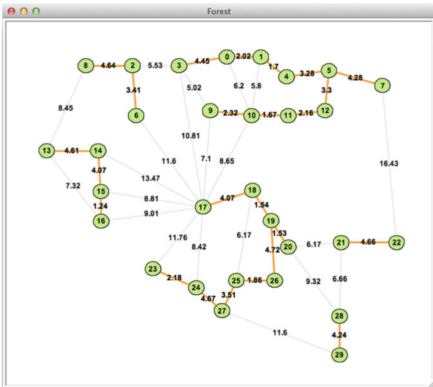
Fig. 7.6 Kruskal's: Snapshot 1
