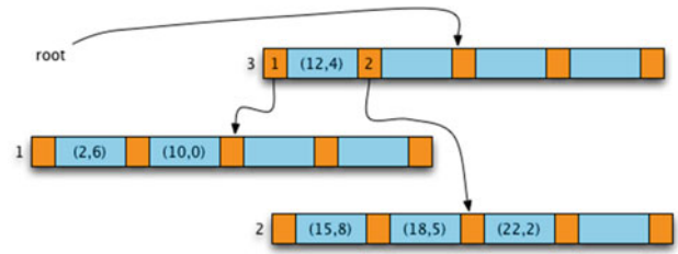
Fig. 11.14 After Deleting the Item Containing 8
