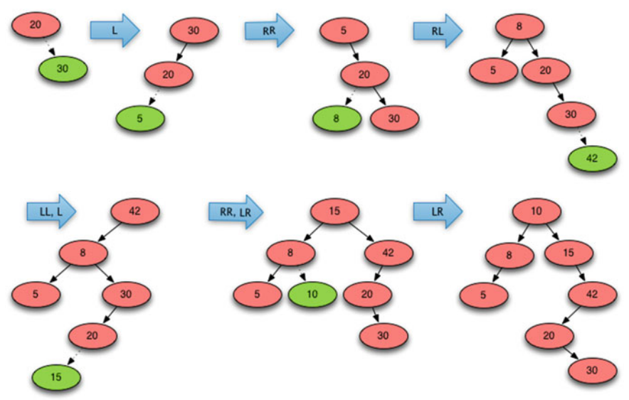
Fig. 10.14 Splay Tree Example
