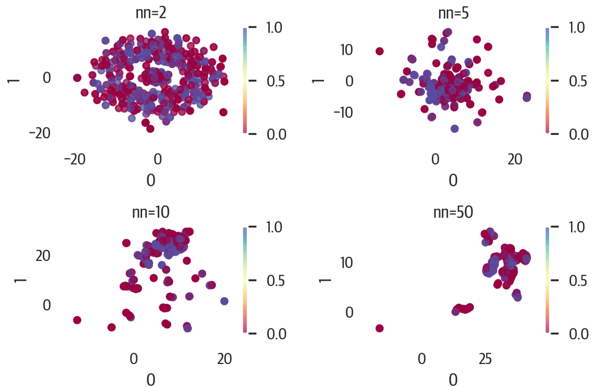
Figure 17-14. UMAP results adjusting n_{\text{neighbors}} .
