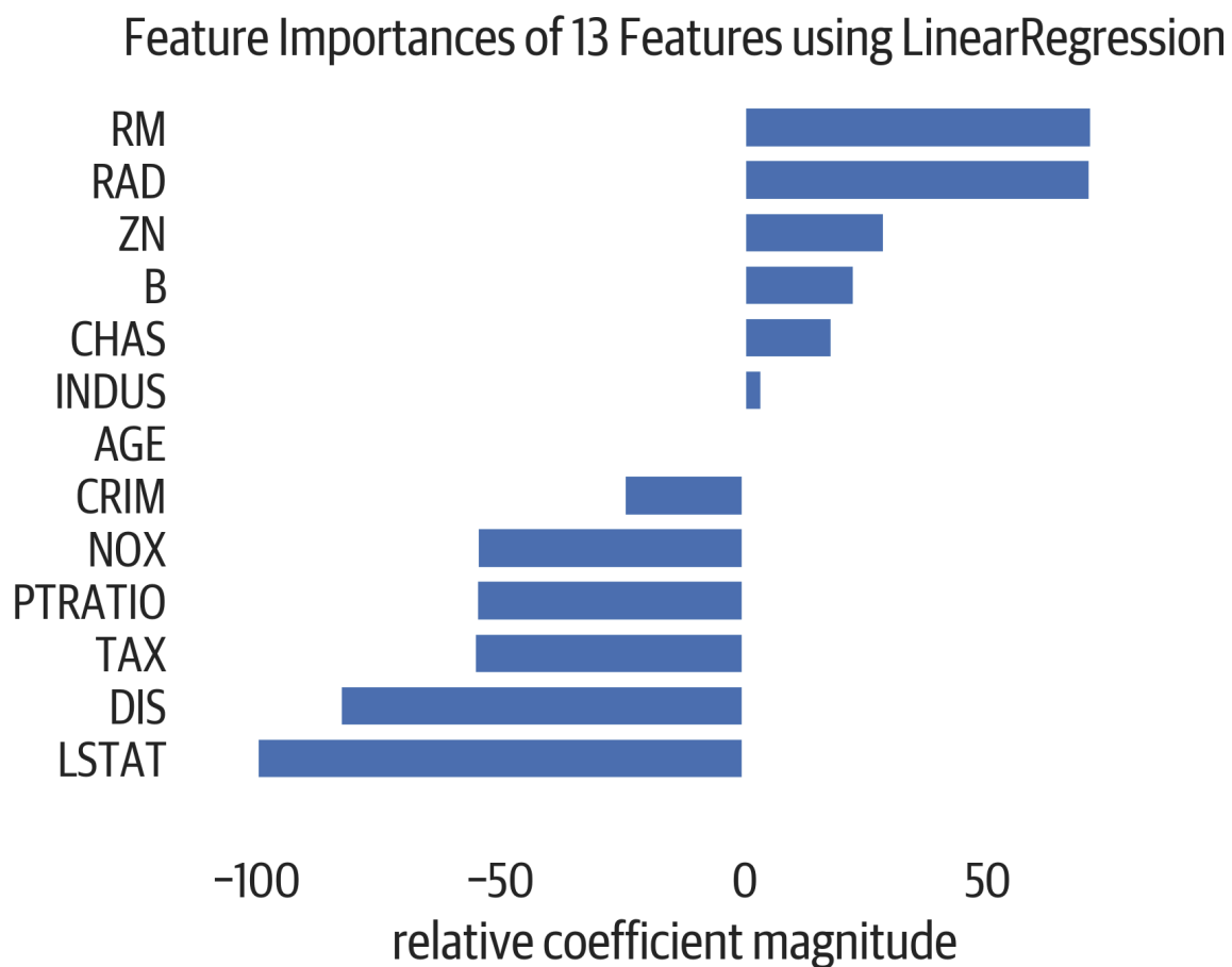
Figure 14-1. Feature importance. This indicates that RM (number of rooms) increases the price, age doesn't really matter, and LSTAT (percent of low status in population) lowers the price.
