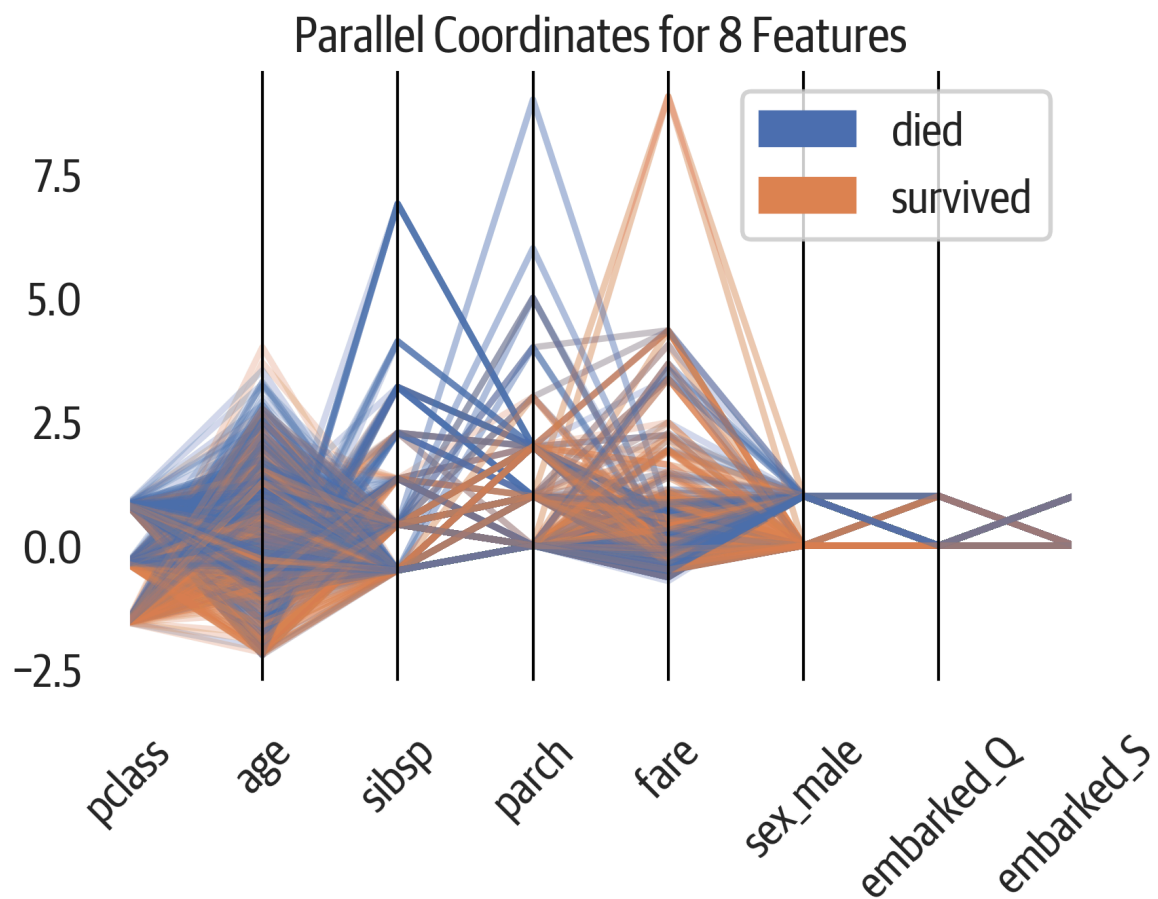
Figure 6-14. Yellowbrick parallel coordinates plot.
