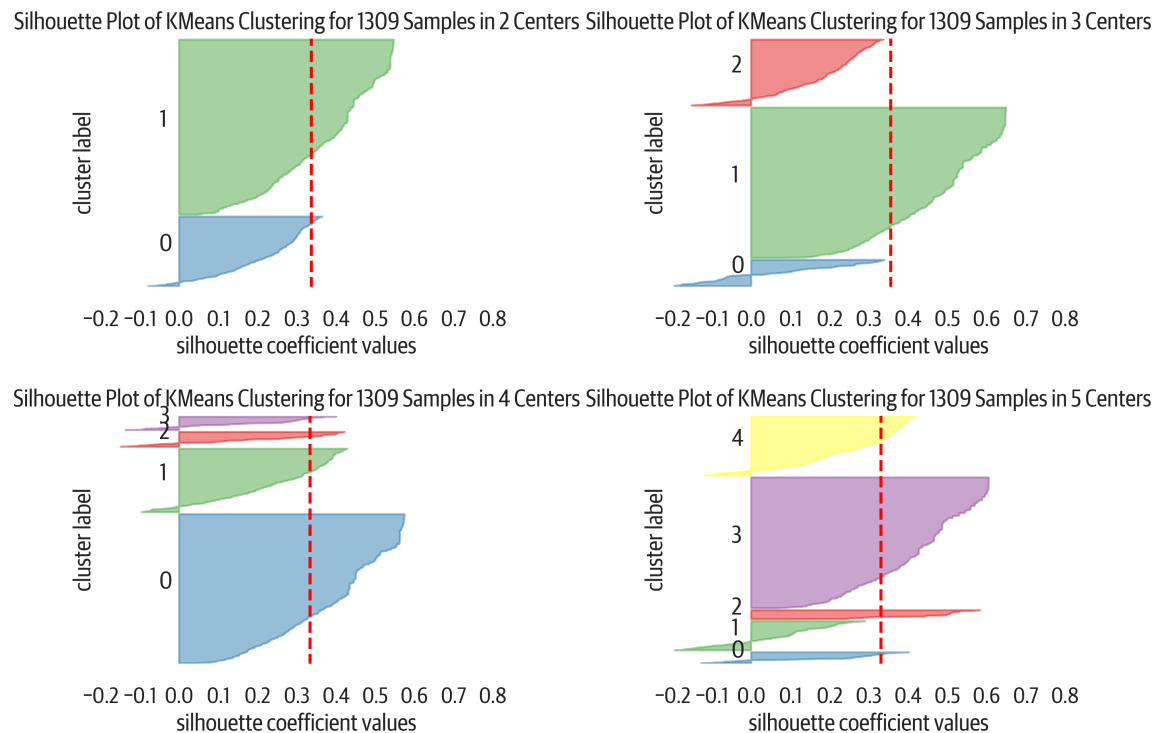
Figure 18-3. Yellowbrick silhouette visualizer
