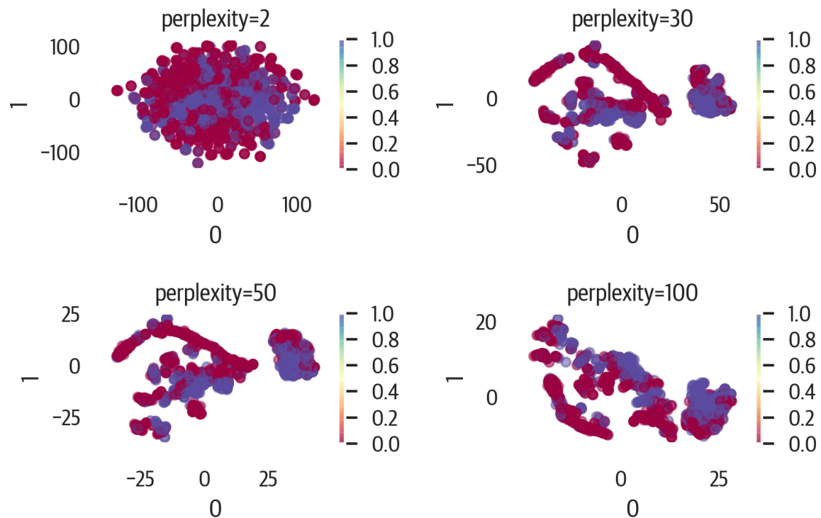
Figure 17-17. Changing perplexity for t-SNE.
